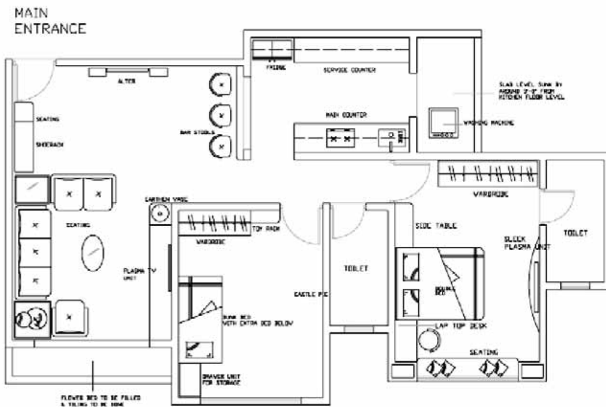
PROPOSED LAYOUT OF MRS.JESSE'S RESIDENCE AT D-ZONE, NEAR GOREGAON FLYOVER, GOREGAON (W)
