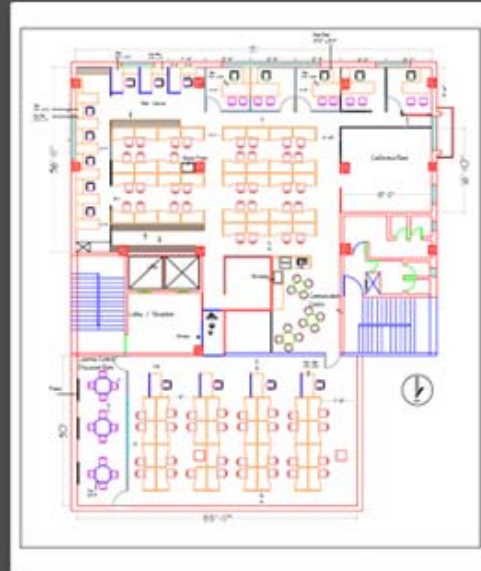
Office Floor layout
